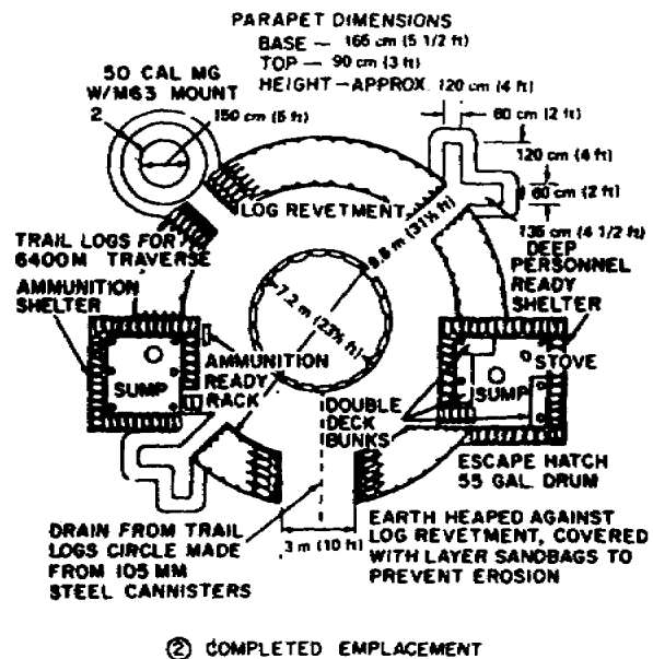
Figure 1-26. Final stage development, howitzer emplacement.
